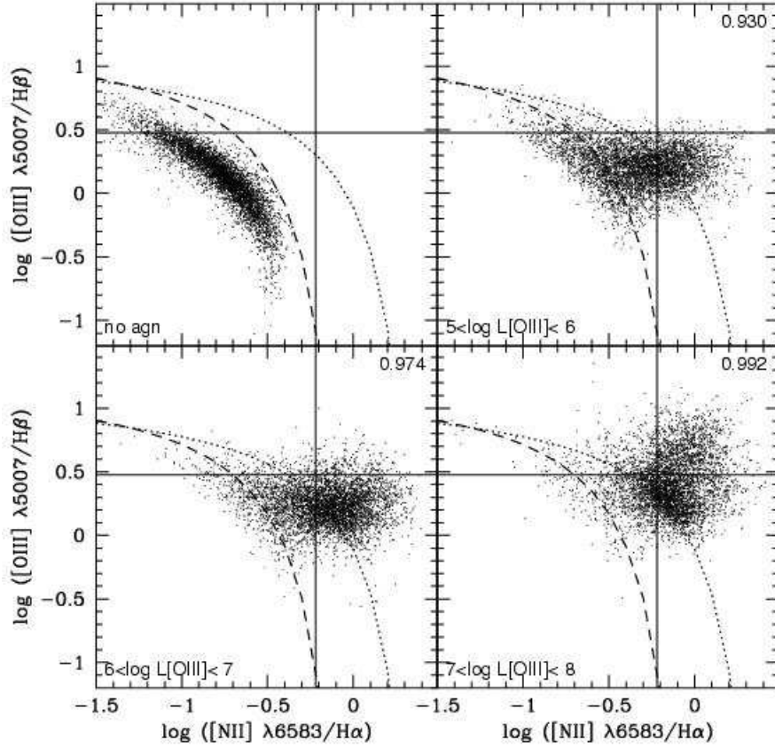
Figure 6: Top left: The BPT diagram of Fig.1 for galaxies with 8 < \log M_* < 9.5 that are not classified as AGN. Next 3 panels: The effect of adding AGN of increasing [OIII] luminosity (see text for more details). The numbers in the upper right corners of each panel indicate the fraction of galaxies that lie above the dashed line.
